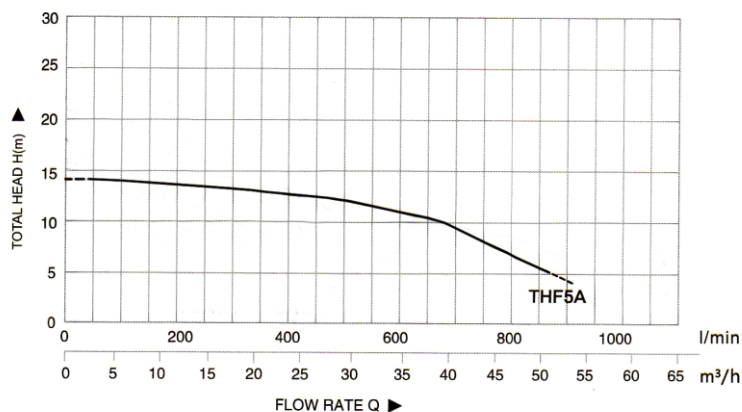
THF 5A Centrifugal Pump
