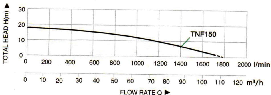
TNF 150 Centrifugal Pump
