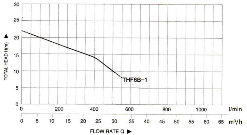
THF 6B - 1 Centrifugal Pump
